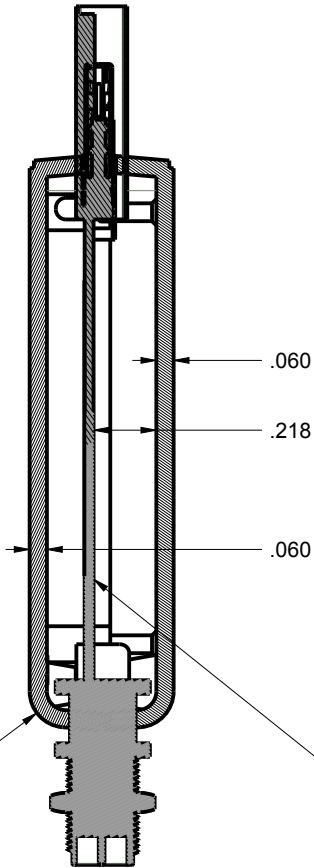
SECTION Y-Y
