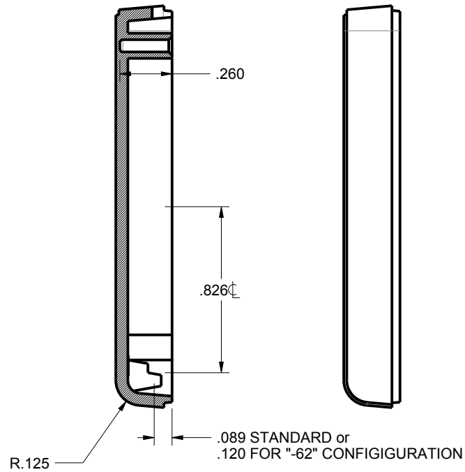
SECTION S-S
