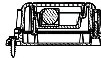
SECTION R-R
