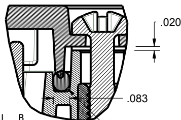
DETAIL B SCALE 2.000
